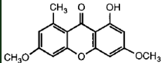
XANTHONE LICHEXANTHONE
