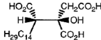
ROCCELLIC ACID
