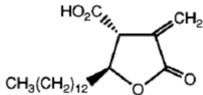
(+)-PROTOLICHESTERINIC ACID
