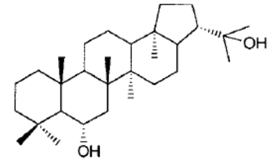
TRITERPENE ZEORIN
