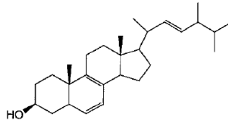
STEROID ERGOSTEROL
